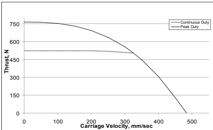
VL-ST60 - SM2316DT @ 42V, 6mm/rev lead ball screw
