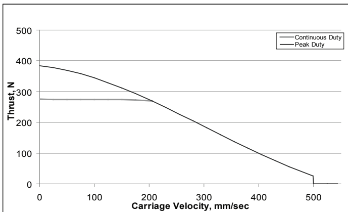
VL-ST45 - SM2316D @ 24V, 6mm/rev lead ball screw
