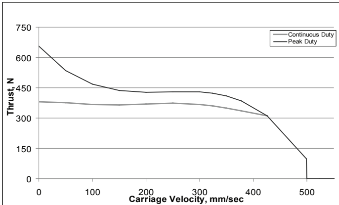
VL-ST45 - SM2315DT @ 48V, 6mm/rev lead ball screw
