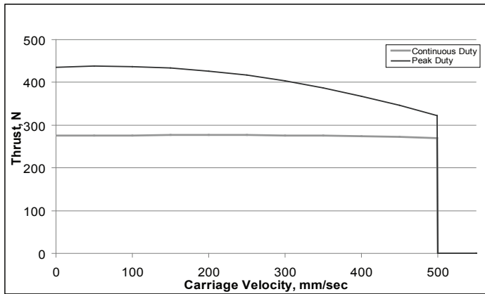
VL-ST45 - SM2316D @ 42V, 6mm/rev lead ball screw
